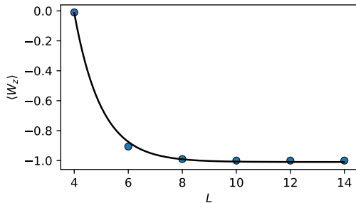
FIG. 3. Final Wilson loop expectation as a function of the system size for sub-critical holding temperature T_{\text{hold}} = 1.2J < T_c and external field B = 0.2J < B_c . The result agrees with a fit \langle W_z \rangle = a \exp(-bL) - 1 , shown in the solid line.
