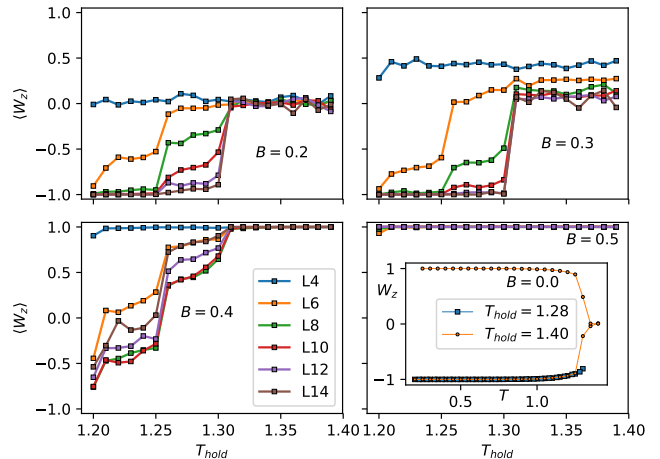
FIG. 2. Expectation value of the Wilson loop \langle W_z \rangle as a function of the holding temperature T_{\text{hold}} for various system sizes and external magnetic fields B . For sufficiently weak external fields and sufficiently low holding temperatures, the system returns to its initial value W_z = -1 with a probability that increases with system size L , suggesting the existence of a self-correcting phase in the (T_{\text{hold}}, B) diagram. At B = 0.4J , we observe that the system of size L = 12 has a higher error probability than L = 10 for all holding temperatures, suggesting that this B exceeds the critical field value. The inset illustrates one typical temperature sweep for two different holding temperatures for a system of size L = 12 . Each data point in the main plots correspond to an average of 1000 such temperature sweeps.
