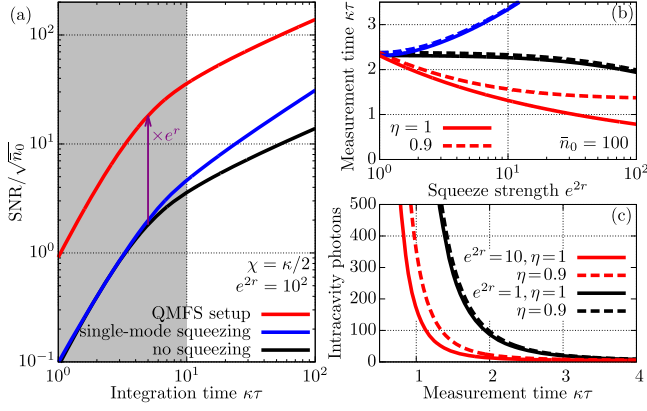
FIG. 3 (color online). (a) SNR as a function of integration time \tau for different protocols: coherent state drive (the black line), displaced single-mode squeezed state (the blue line), two-mode squeezed QMFS setup (the red line). We assume an optimal dispersive shift \chi = \kappa/2 ; for the QMFS setup, the cavity is presqueezed ( t_0 \ll -1/\kappa ) with squeeze strength e^{2r} = 100 . The coherent drive is turned on at \tau = 0 . For the single-mode case, for each \tau we optimize the squeeze strength e^{2r} \in [1, 100] and angle (see Ref. [25]). The QMFS scheme gives an exponential SNR enhancement, especially in the most interesting regime where \tau \sim 1/\kappa (the shaded region). (b) Integration time \tau required to achieve a fidelity F = 99.99\% , as a function of e^{2r} ; parameters as in (a), except that \bar{n}_0 = 100 . Black lines correspond to an unsqueezed drive, where the drive strength is increased such that the intracavity photon number is the same as in the QMFS scheme, i.e., \bar{n}_0 \rightarrow \bar{n}_0 + 4 \sinh^2 r . The solid curves correspond to the case of no photon losses (efficiency \eta = 1 ), while the dashed curves correspond to \eta = 0.9 . (c) Total intracavity photon number needed to achieve F = 99.99\% in a measurement time \tau . Even with nonzero photon losses, the use of squeezing can dramatically reduce the number of intracavity photons.
