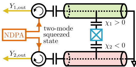
FIG. 2 (color online). Circuit QED implementation of QMFS dispersive qubit read-out with two-mode-squeezed states produced by a nondegenerate paramp (NDPA). The signal is encoded in the joint quadrature Y_{+,out} \propto Y_{1,out} + Y_{2,out} ; see the text for details.
