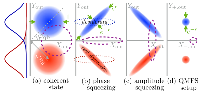
FIG. 1 (color online). Phase-space representation of dispersive qubit read-out for different input states: (a) coherent state, (b) single-mode phase-squeezed state, (c) amplitude-squeezed state, (d) two-mode squeezed state in the QMFS ( X_- , Y_+ ). The purple dashed lines represent the input state and the blobs represent the output fields. The input state is displaced along the X axis and the signal is encoded in the quadrature corresponding to the Y axis with homodyne detection; as depicted in the leftmost panel, the read-out error corresponds to the overlap of the two marginals. Dispersive interaction with the qubit rotates the output field by the angle \varphi_{qb} for the ground state |0\rangle (in blue) and -\varphi_{qb} for the excited state |1\rangle (in red). Ideally, one wants the output state to be phase squeezed regardless of qubit state [the dotted “desiderata” states in (b)]; this is not possible when using single-mode squeezing due to the qubit-induced rotation. Our new QMFS scheme [panel (d)] does not suffer from this problem.
