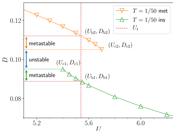
FIG. 11. Double occupancy D versus U at T = 1/50 < T_c . Spinodal points and binodal points are indicated. Vertical arrows denote the metastable regions and the unstable region.
