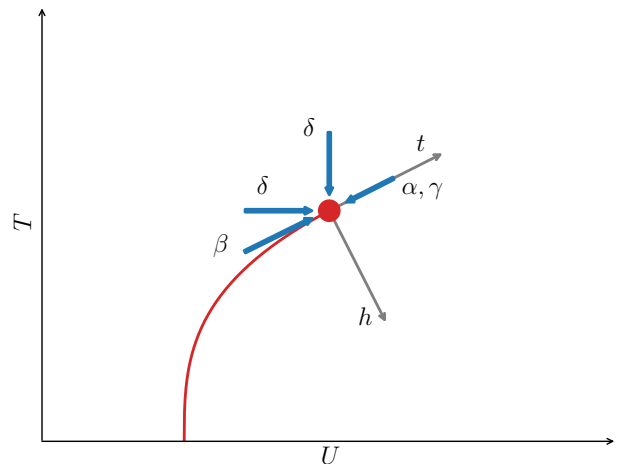
FIG. 15. Sketch of the interaction-driven Mott transition in the T - U plane. The first-order transition (continuous red line) terminates in a second-order endpoint at (U_c, T_c) (red circle). Gray arrows indicate the eigendirections t and h . Blue arrows indicate the critical exponents along directions of interest here.
